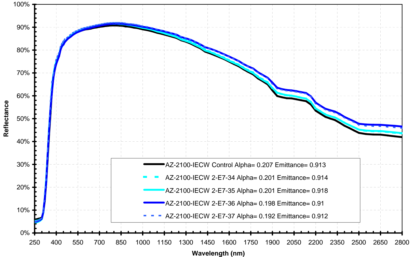
Post-Flight MISSE AZ Electrically Conductive White Coating: AZ-2100-IECW
