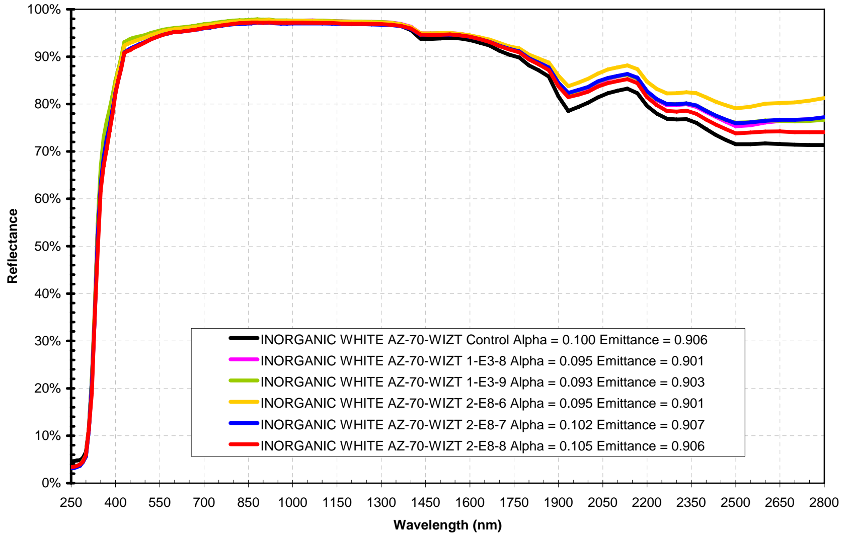
Post-Flight MISSE AZ-70-WIZT Inorganic White Thermal Control Coating
