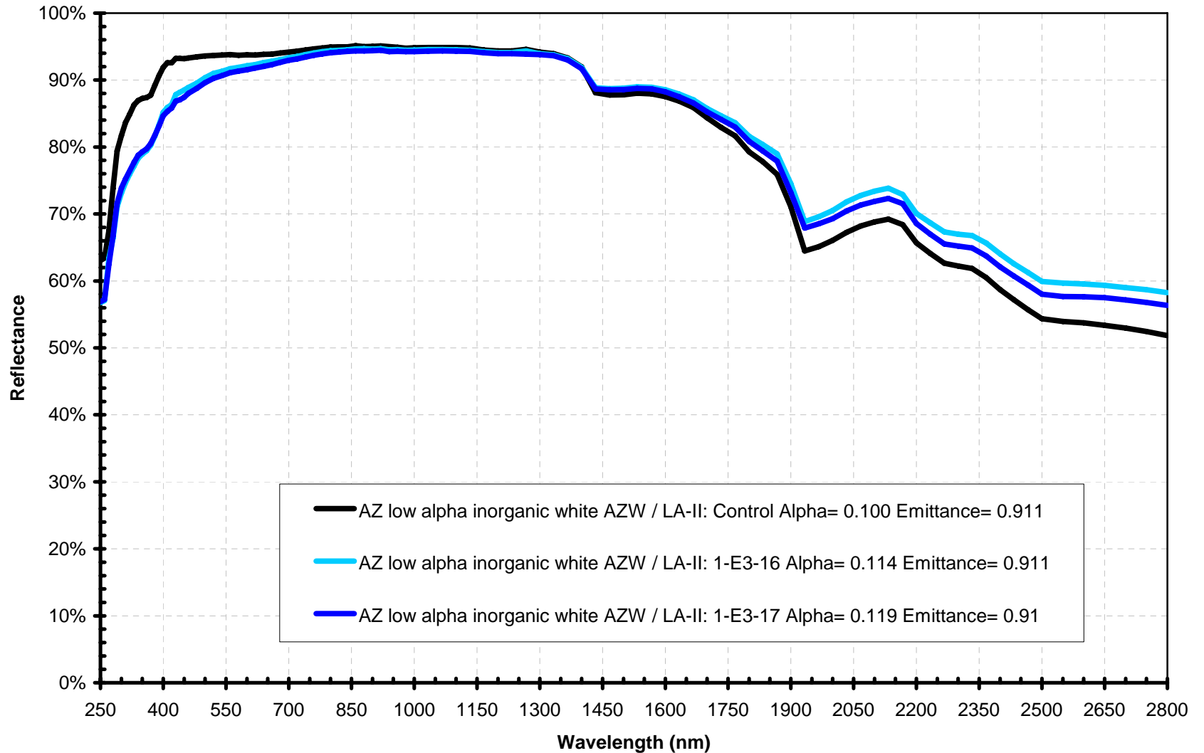
Post-Flight MISSE AZ Inorganic White Low Alpha Thermal Control Coating: AZW / LA-II
